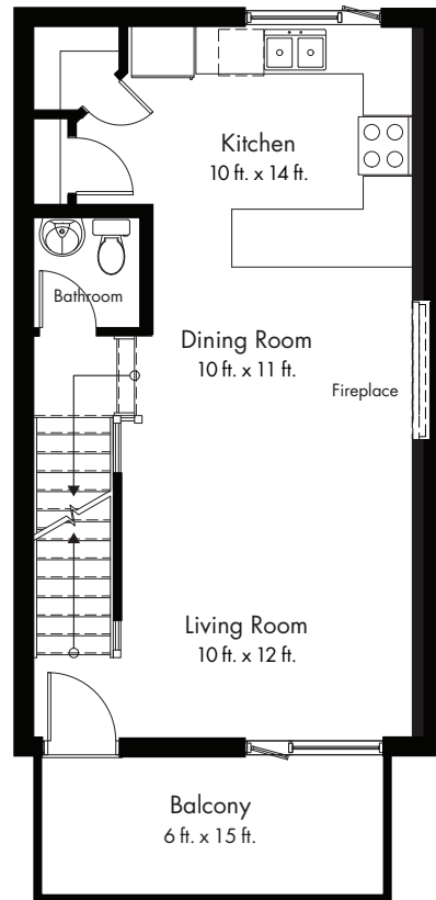
Main Floor: 586 S.F.
