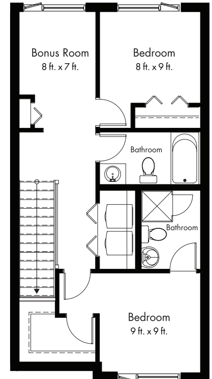
Upper Floor Alt: 633 S.F.
